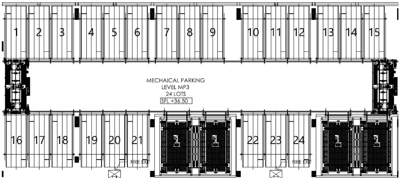
SAMPLE PARKING FLOOR PLAN
