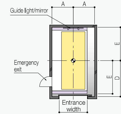
Plan view of standard-type boarding area
