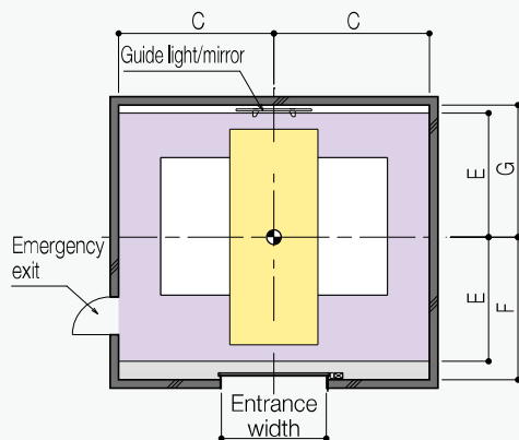
Plan view of the boarding area with turntable (90° type)
