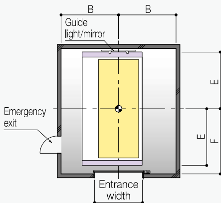
Plan view of the boarding area with turntable (180° type)
